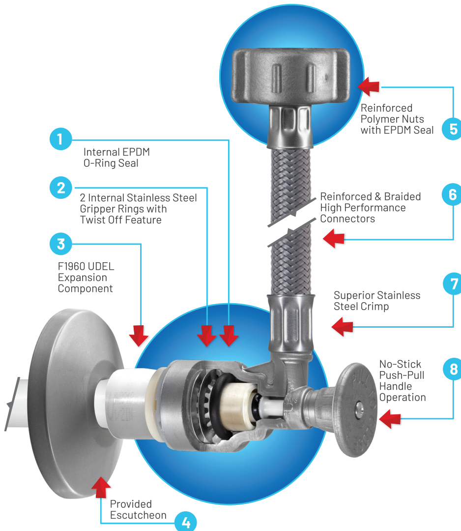
INSTALLED VALVE
